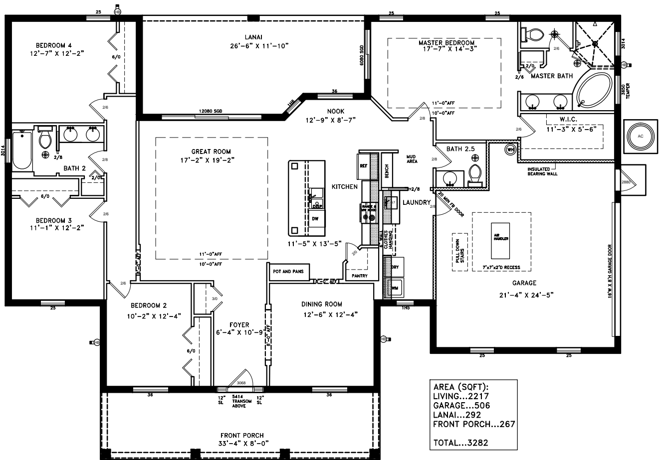
THE OCALA (73'-4"W X 53'-0"D) © COPYRIGHT TRINITY DRAFTING LLC
